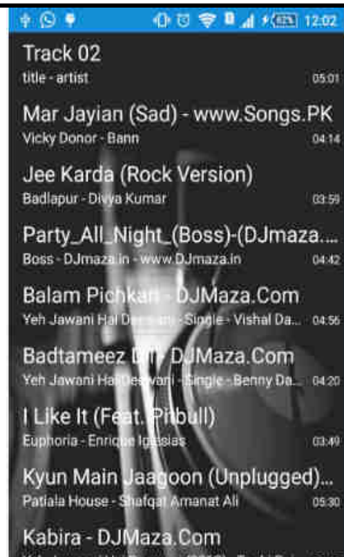
Fig 8: Xbeats UI
