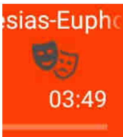
Fig 9: SenseMe button
